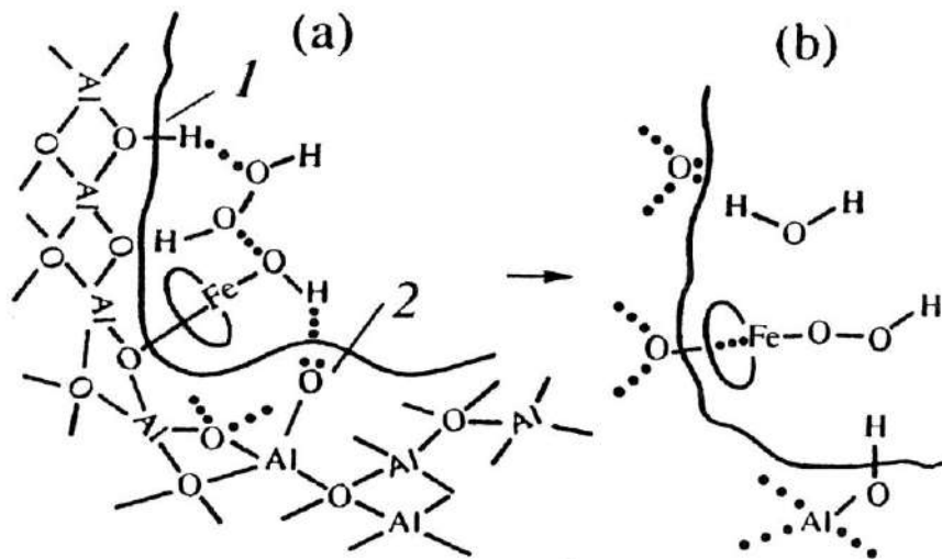
Fig. 3. The mechanism of catalyst-substrate complex formation: (a) formation of active complex with participation of acid-base centers of \text{Al}_2\text{O}_3 ; (b) active intermediate, catalyst-substrate complex; (1) acid center; (2) base center; points are forming bonds; solid lines are breaking bonds.
