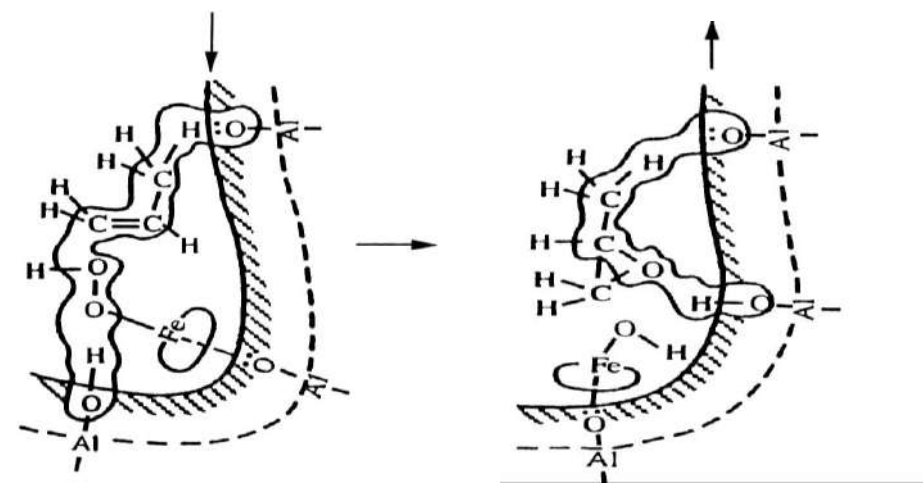
Fig. 4. The mechanism of propylene oxide formation on the per-FTPhPFe(III)OH/ \text{Al}_2\text{O}_3 .
